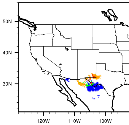
Diff (A2-Mod) yucctorr
