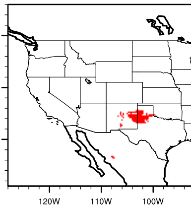
IPSL future yucctorr
