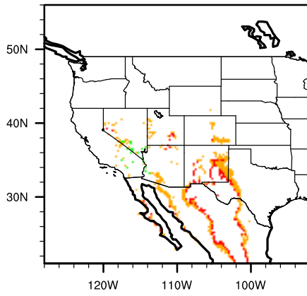
Diff (A2-Mod) yuccfaxo
