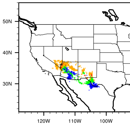
Diff (A2-Mod) yuccelat
