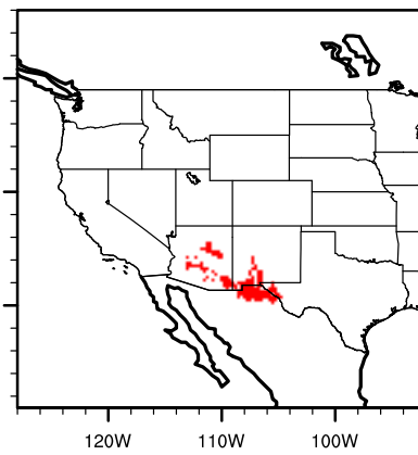
IPSL future yuccelat
