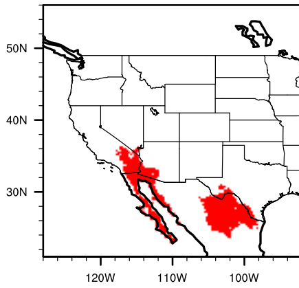
Diff (A2-Mod) yuccarn
