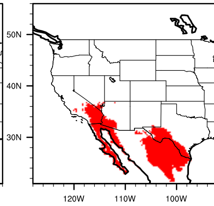
IPSL future yuccarn
