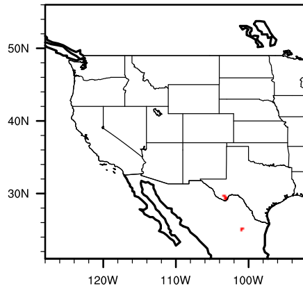
Model modern yuccarn
