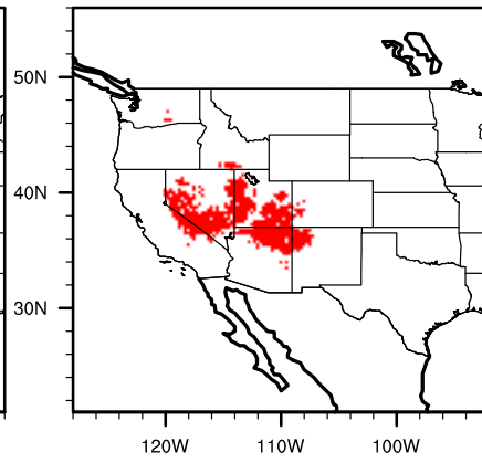
IPSL future yuccabrev
