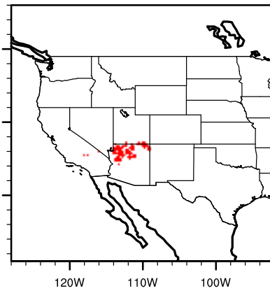
IPSL future yuccabrev
