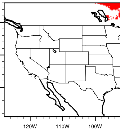
IPSL future ulmuamer
