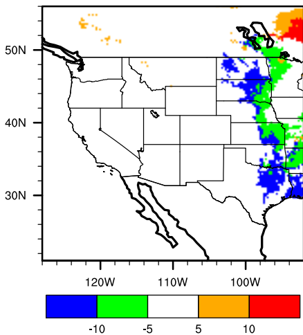
Diff (A2-Mod) ulmuamer
