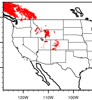
IPSL future sorbscop
