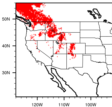
Model modern sorbscop
