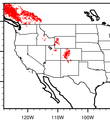
PCM1 future sorbscop
