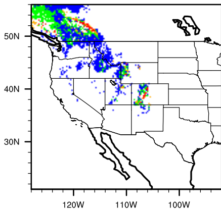
Diff (A2-Mod) sorbscop
