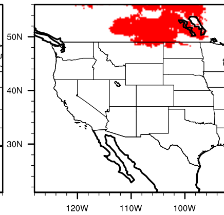
IPSL future sheparge
