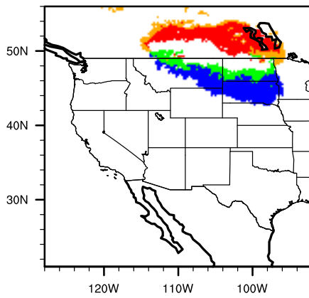
Diff (A2-Mod) sheparge
