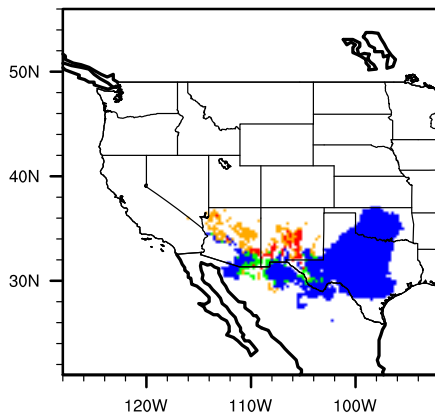
Diff (A2-Mod) sapidrum
