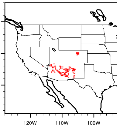
IPSL future sapidrum
