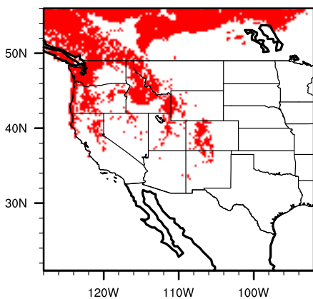
Model modern saliscou
