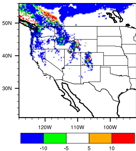
Diff (A2-Mod) saliscou
