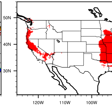
IPSL future salinigr
