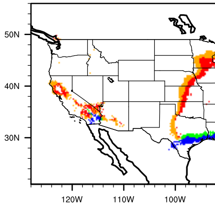
Diff (A2-Mod) salinigr
