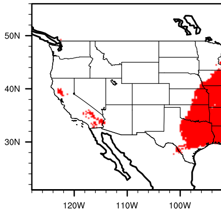
Model modern salinigr
