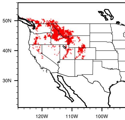
Diff (A2-Mod) saligege
