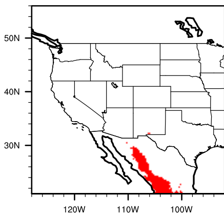
Model modern salibonp
