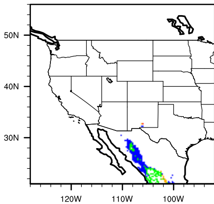
Diff (A2-Mod) salibonp
