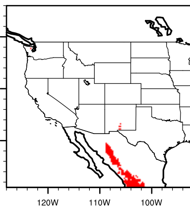
PCM1 future salibonp
