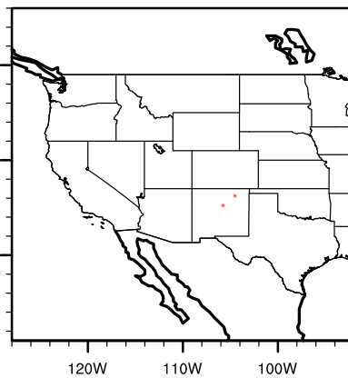
IPSL future salibonp
