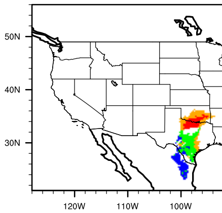
Diff (A2-Mod) rhuslanc
