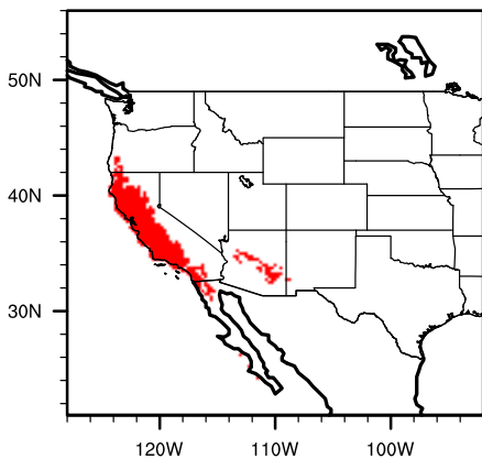
Model modern rhamcali
