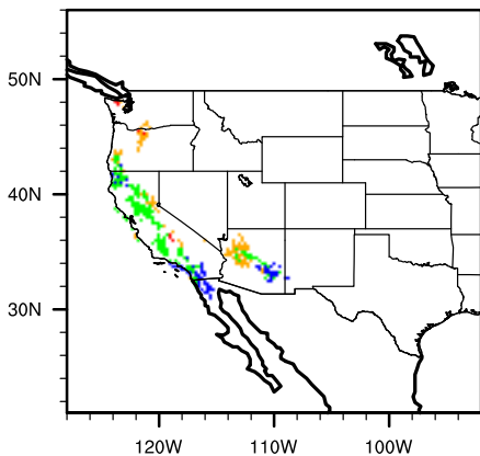
Diff (A2-Mod) rhamcali
