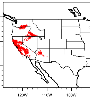
IPSL future rhamcali
