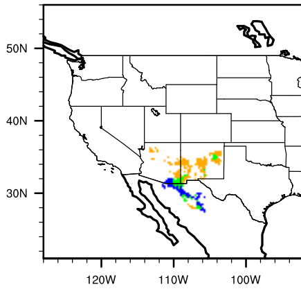
Diff (A2-Mod) querhypo
