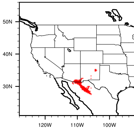
Model modern querhypo
