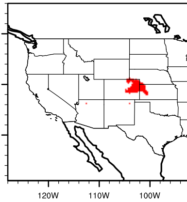
IPSL future querhypo
