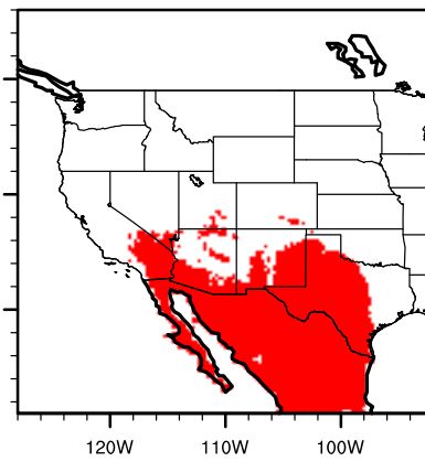
IPSL future quergrav
