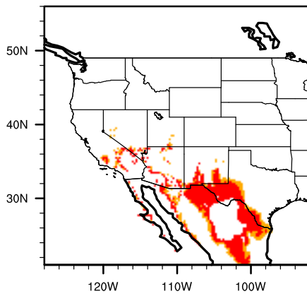
Diff (A2-Mod) quergrav
