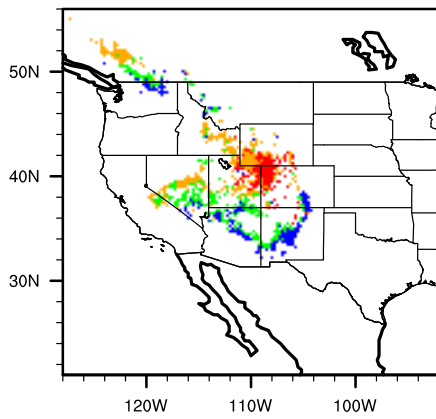
Diff (A2-Mod) quergamb
