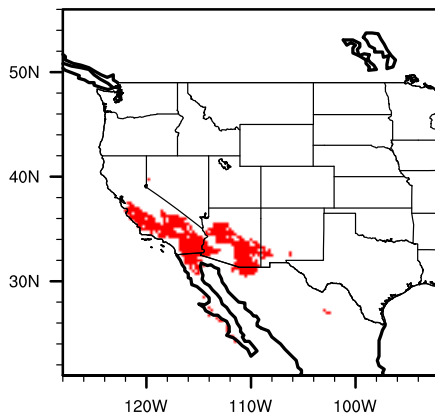
Diff (A2-Mod) querdunn
