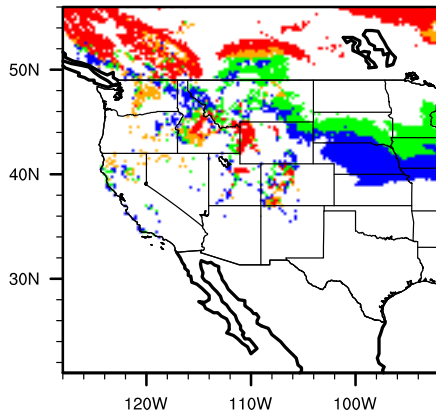
Diff (A2-Mod) prunvirg
