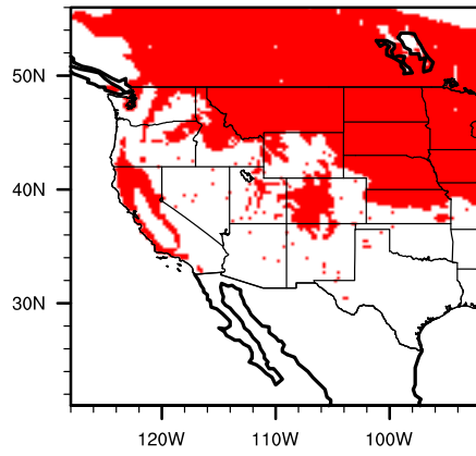
Model modern prunvirg
