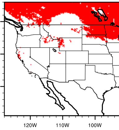
IPSL future prunvirg
