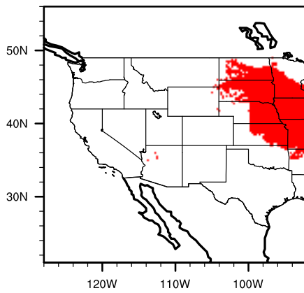
Diff (A2-Mod) prunamer
