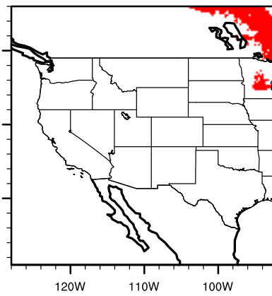
IPSL future prunamer
