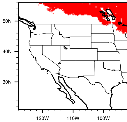
Diff (A2-Mod) popubals
