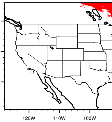
IPSL future popubals
