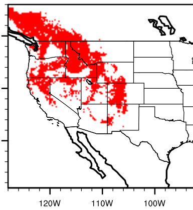
IPSL future pinupond
