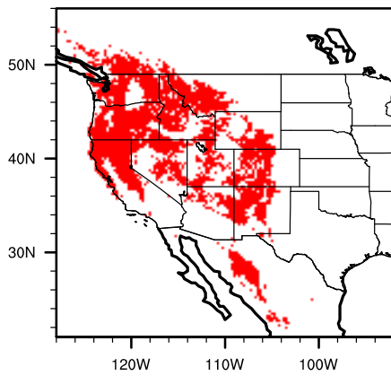
Diff (A2-Mod) pinupond
