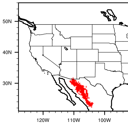
Diff (A2-Mod) pinuenge
