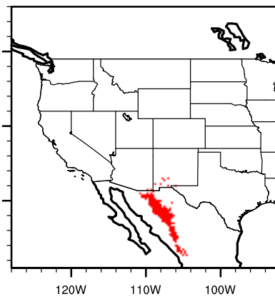
IPSL future pinuenge
