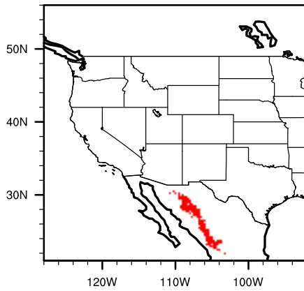
Model modern pinudura
