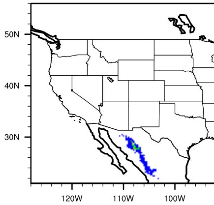
Diff (A2-Mod) pinudura
