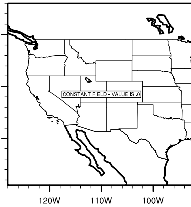
IPSL future pinudura
