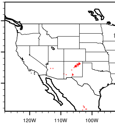
IPSL future pinucemb
