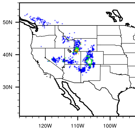
Diff (A2-Mod) picepung
