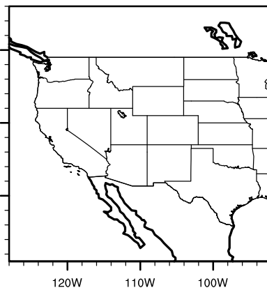
IPSL future lysimicr
