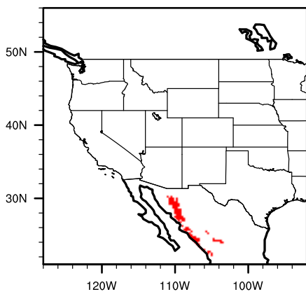
Model modern lysimicr
