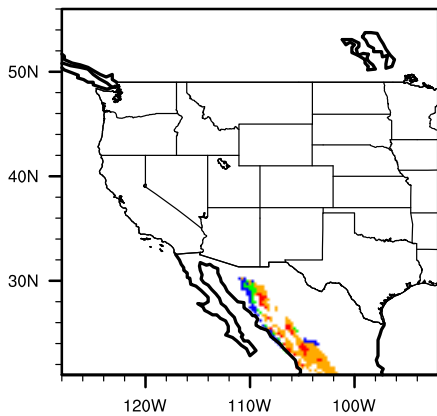
Diff (A2-Mod) lysimicr
