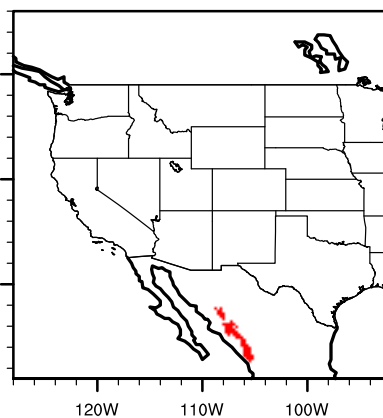
IPSL future leucretu
