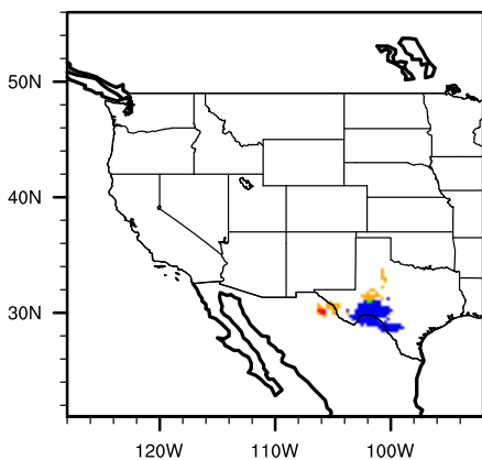
Diff (A2-Mod) leucretu
