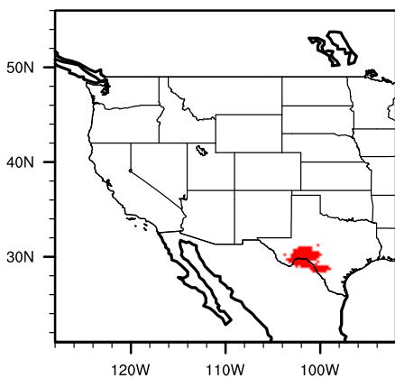
Model modern leucretu
