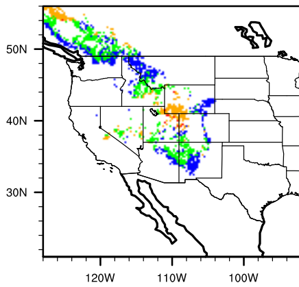
Diff (A2-Mod) juniscop
