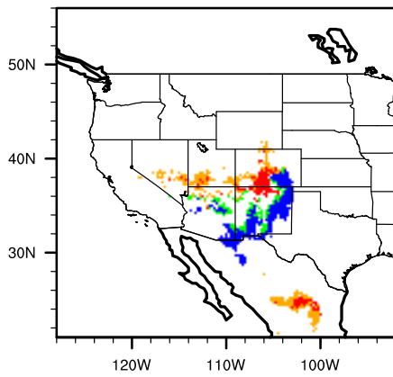
Diff (A2-Mod) junimono
