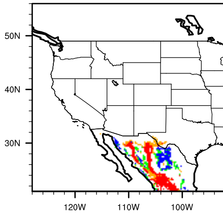
Diff (A2-Mod) juniflac
