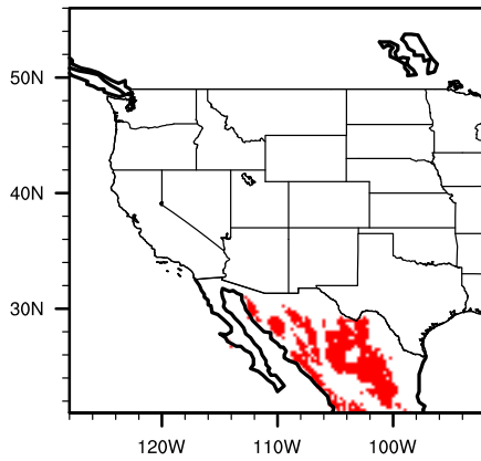
Model modern juniflac
