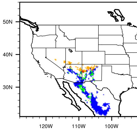
Diff (A2-Mod) junidepp
