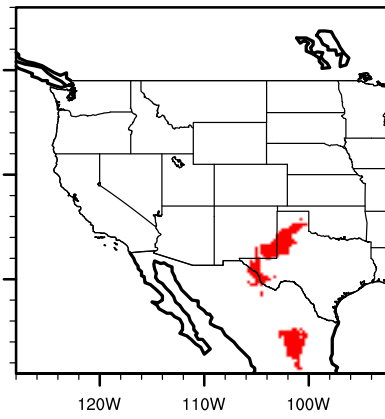
IPSL future juglmicr
