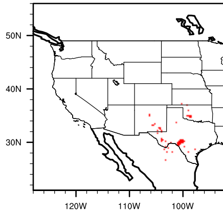
Model modern juglmicr
