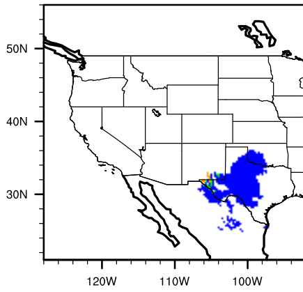
Diff (A2-Mod) juglmicr
