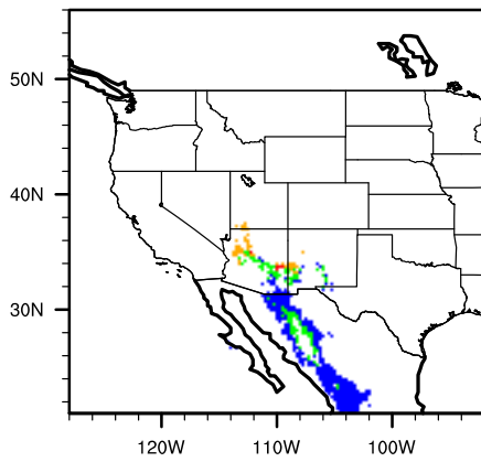
Diff (A2-Mod) juglmajo
