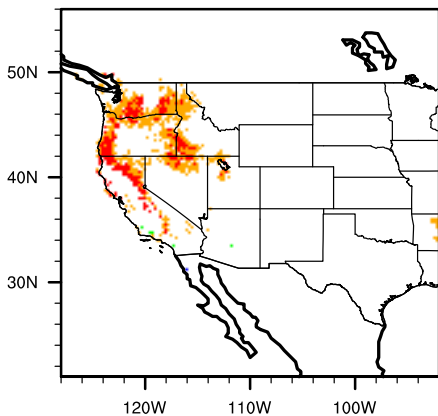
Diff (A2-Mod) fremcali
