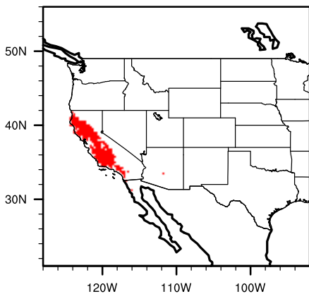
Model modern fremcali
