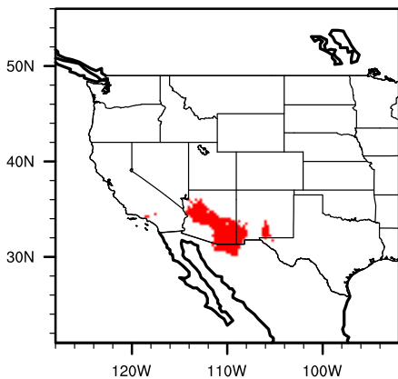
Model modern fraxvelu
