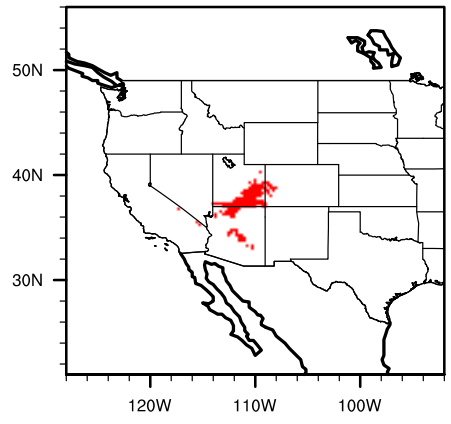
Model modern fraxanom
