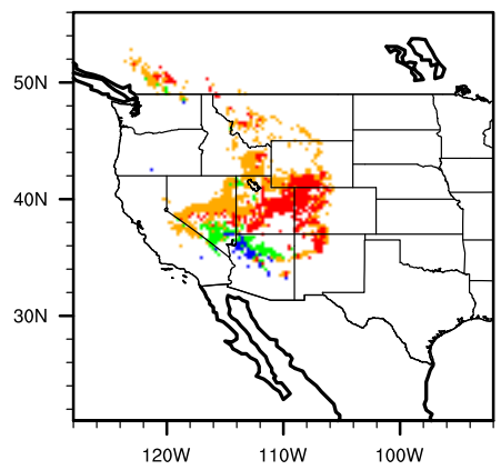
Diff (A2-Mod) fraxanom
