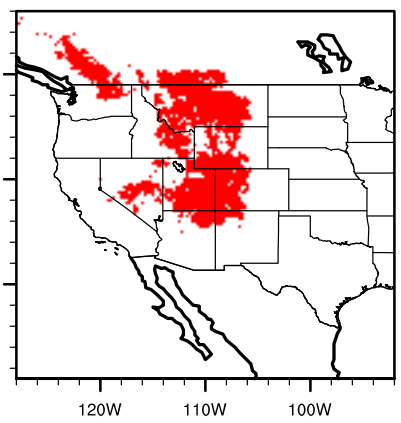
IPSL future fraxanom
