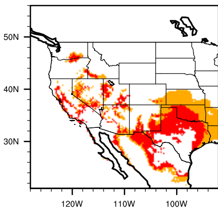
Diff (A2-Mod) cratrac
