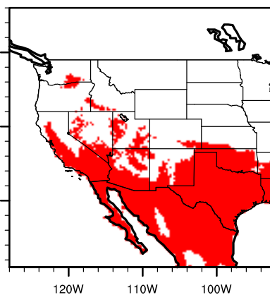
IPSL future cratrac
