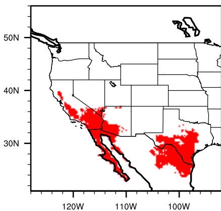
Model modern cratrac
