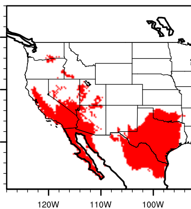
PCM1 future cratrac
