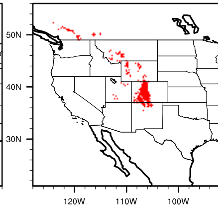
IPSL future crateryt
