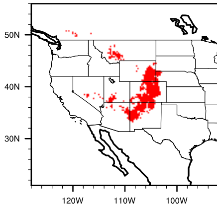
Diff (A2-Mod) crateryt
