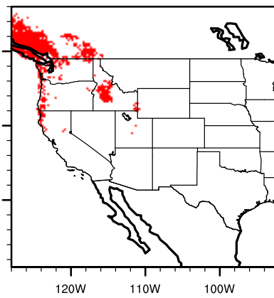
IPSL future cratdoug
