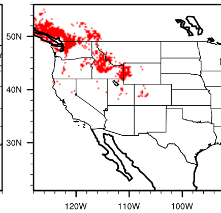
IPSL future cratdoug
