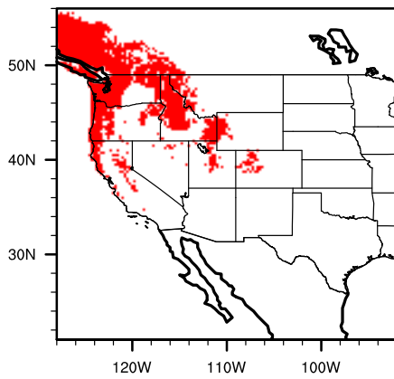
Diff (A2-Mod) cratdoug
