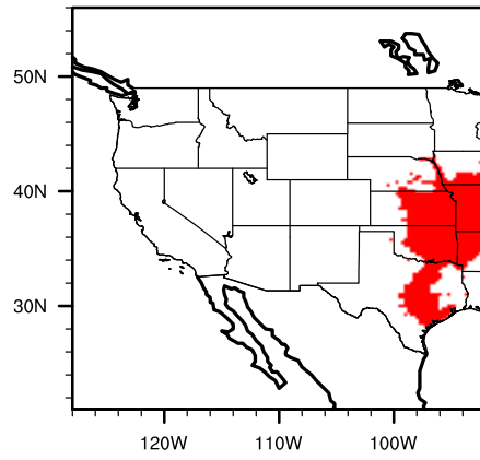
Model modern corndrum
