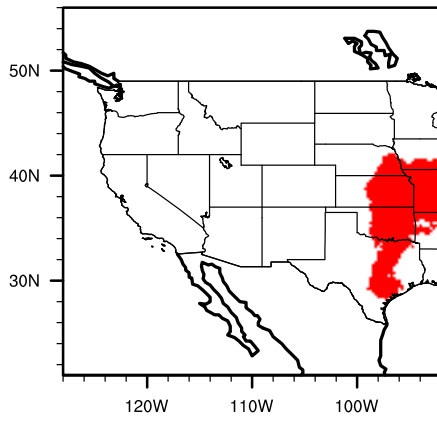
Diff (A2-Mod) corndrum
