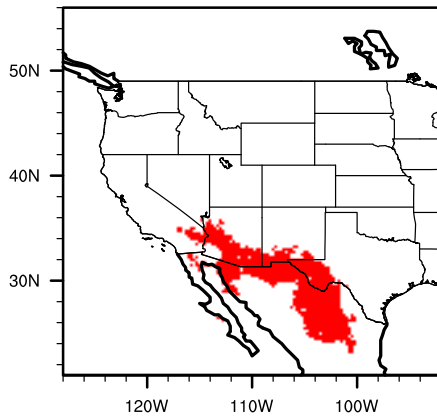
Diff (A2-Mod) chilline
