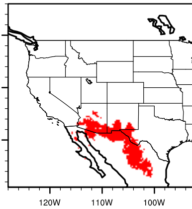
IPSL future chilline
