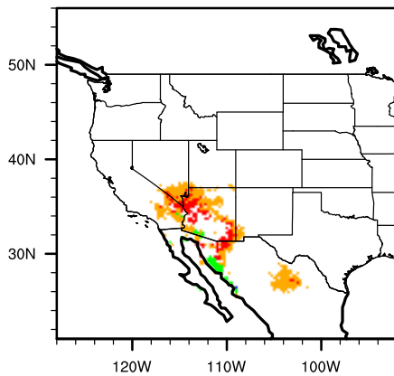
Diff (A2-Mod) ceregiga
