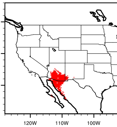
IPSL future ceregiga
