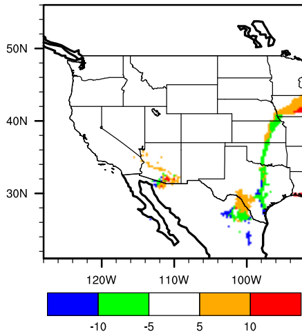
Diff (A2-Mod) cerccana
