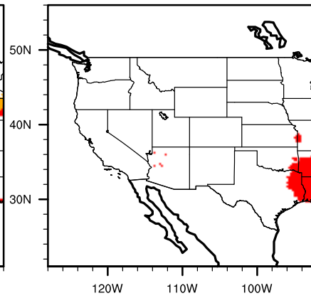
IPSL future cerccana
