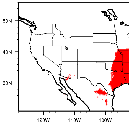
Diff (A2-Mod) cerccana
