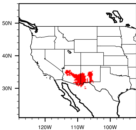
Model modern cercbrev
