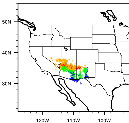
Diff (A2-Mod) cercbrev
