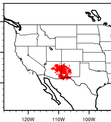
PCM1 future cercbrev
