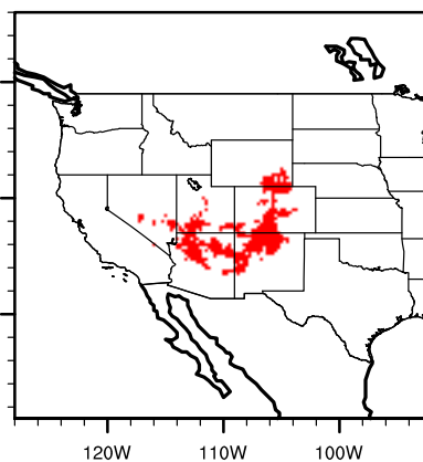
IPSL future cercbrev
