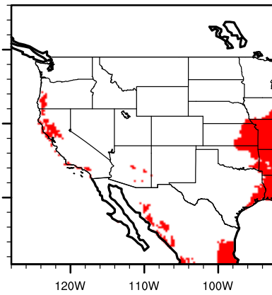
PCM1 future cephocci
