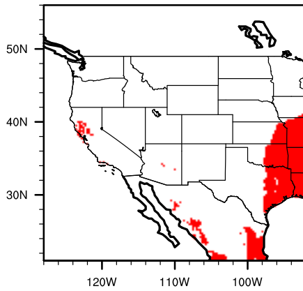
Model modern cephocci
