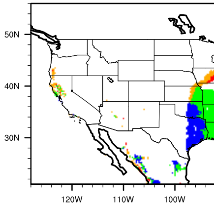
Diff (A2-Mod) cephocci
