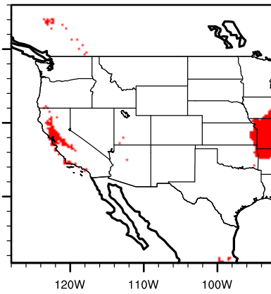
IPSL future cephocci
