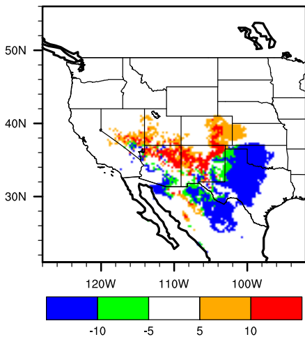
Diff (A2-Mod) celtreti
