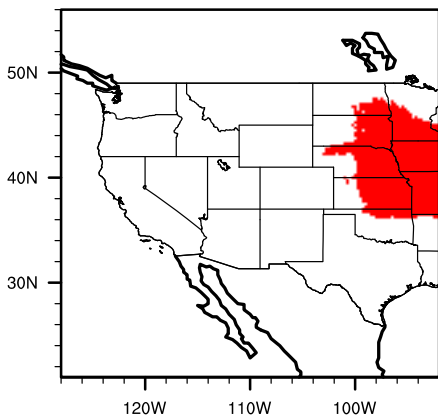
Diff (A2-Mod) celtocci
