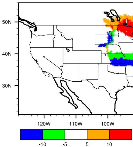
Diff (A2-Mod) celtocci
