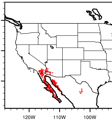
IPSL future bursmicr
